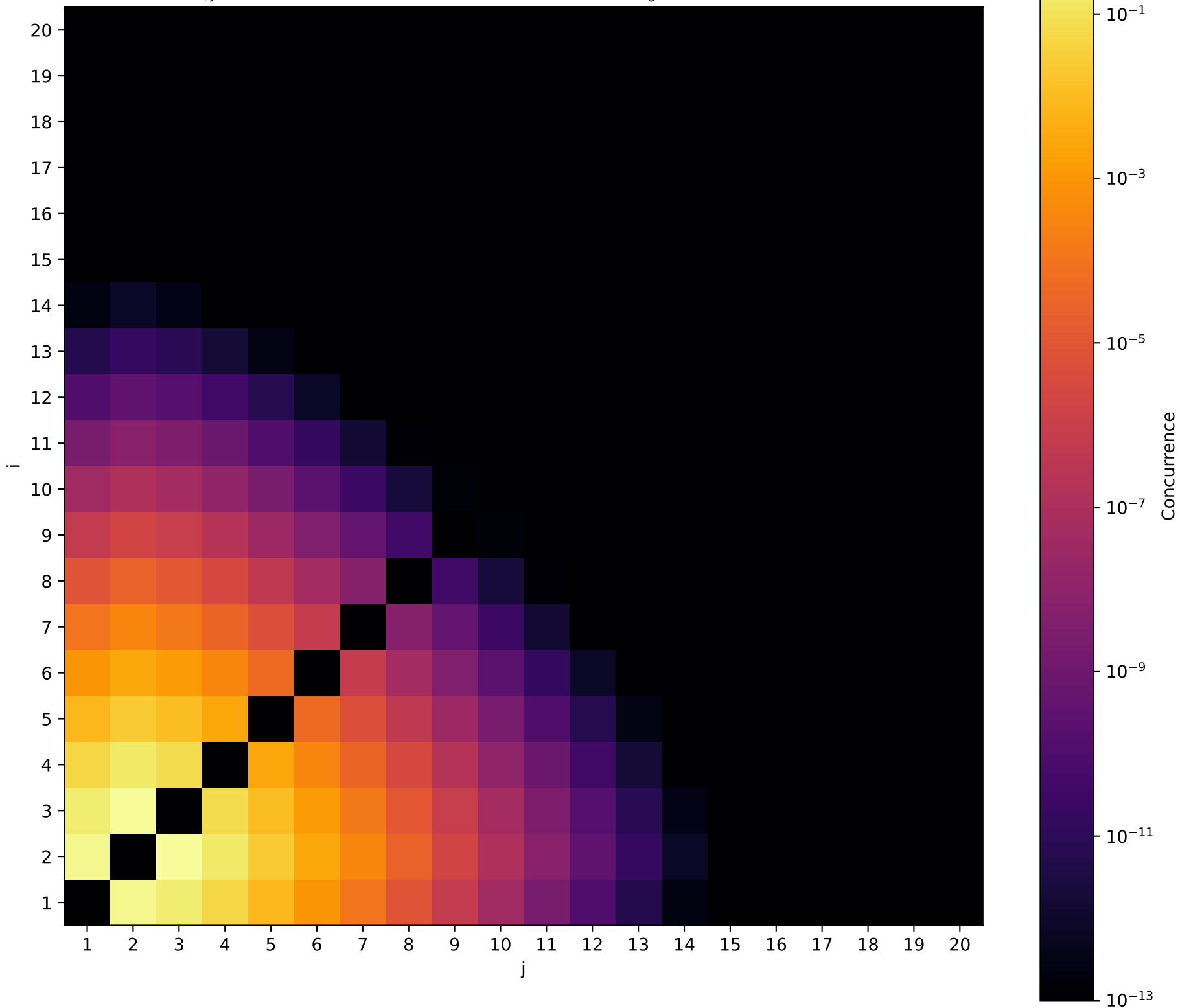
C_{i,j}(t = t : .2f) for prod state (2) (band 1) - J_{long} = 20, J_z = 1, \alpha = 0.5
